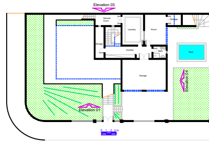
Lower Floor Plan A = 121,28 m 2
