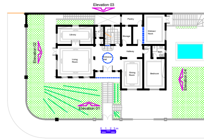
First Floor Plan A = 178,43 m 2
