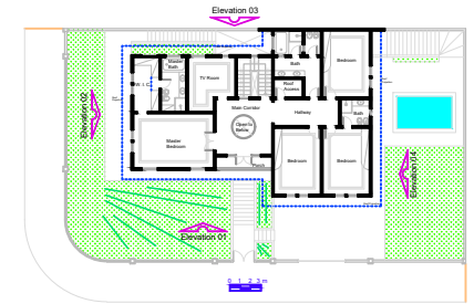
Second Floor Plan A = 181,02 m 2
